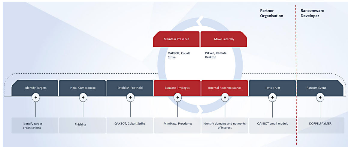
Figure 3: The QAKBOT and Doppelpaymer partnership in the ransomware attack life cycle
